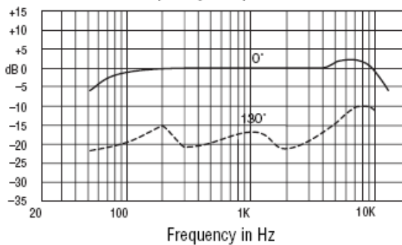
Frequency Response
