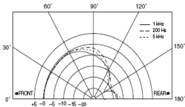
Vertical-Plane Polar Response
