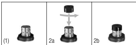
Fig. 4: Microphone capsule without (1) and with (2b) PB 1000.
